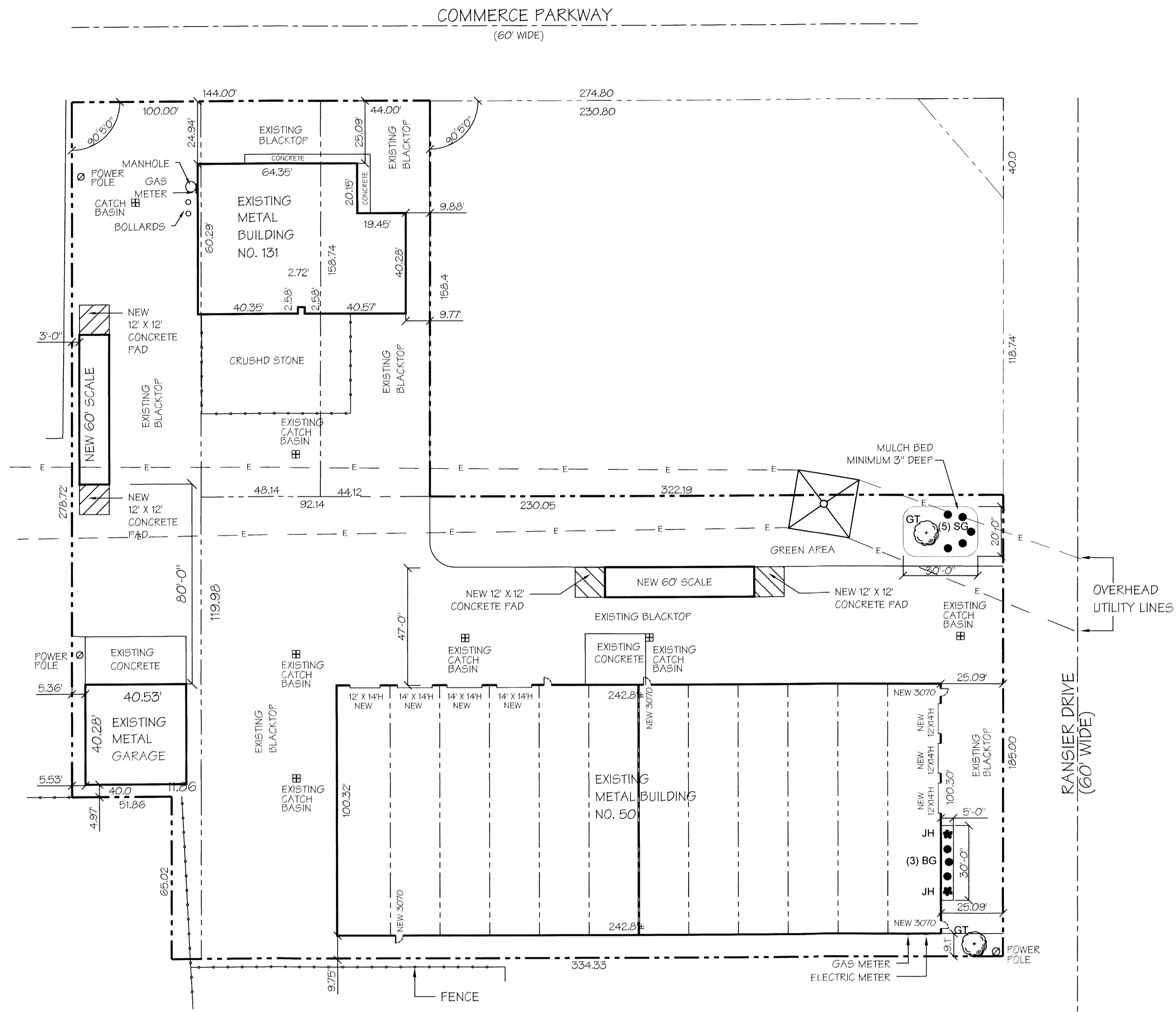
SITE PLAN SCALE: 1" = 30'-0"
