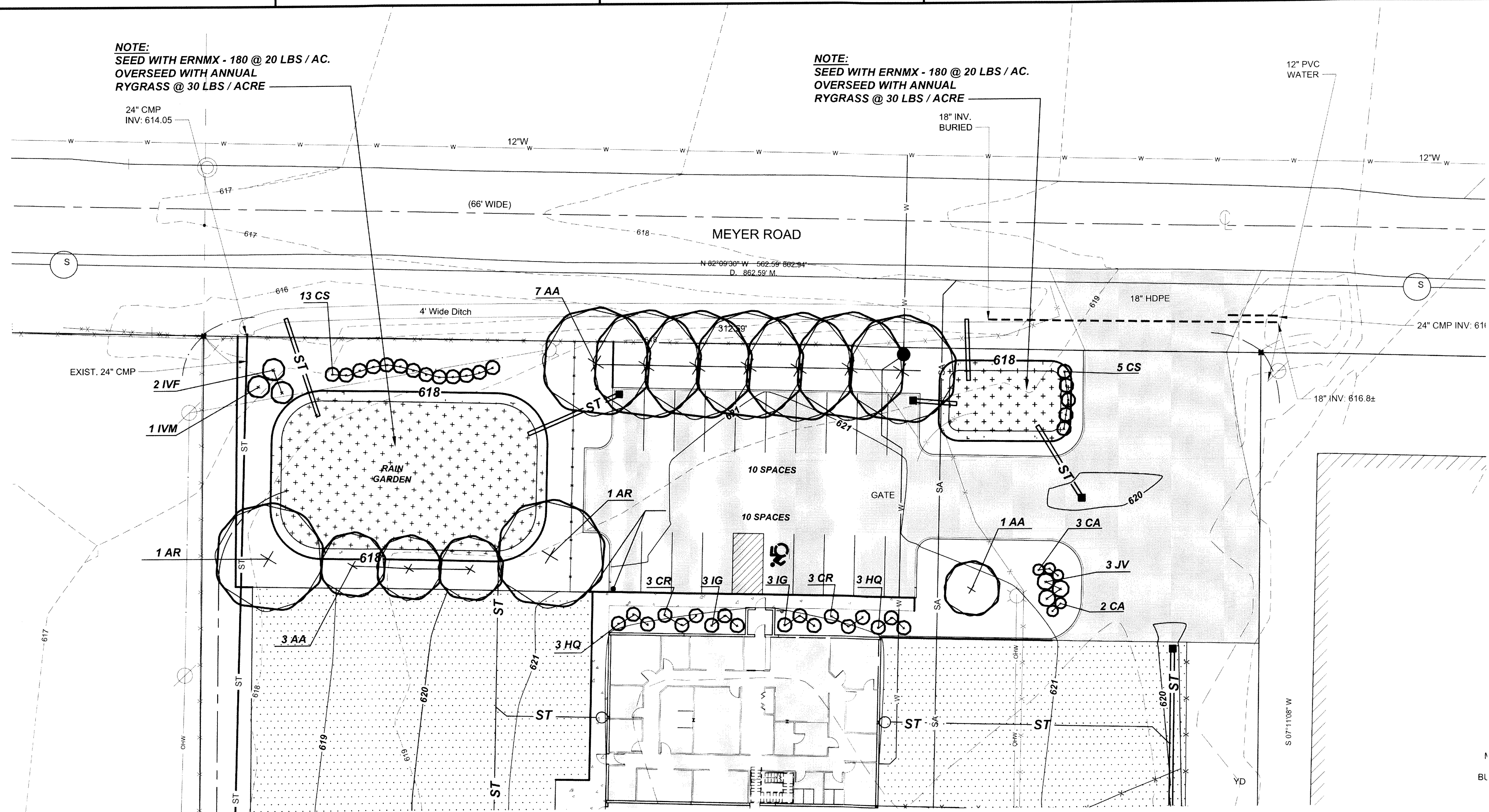
1 LANDSCAPING PLAN SCALE: 1"=20'
