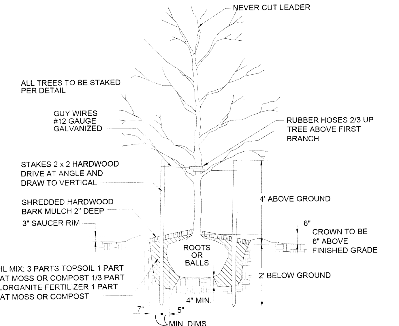
2 DECIDUOUS TREE PLANTING SCALE: NO SCALE
