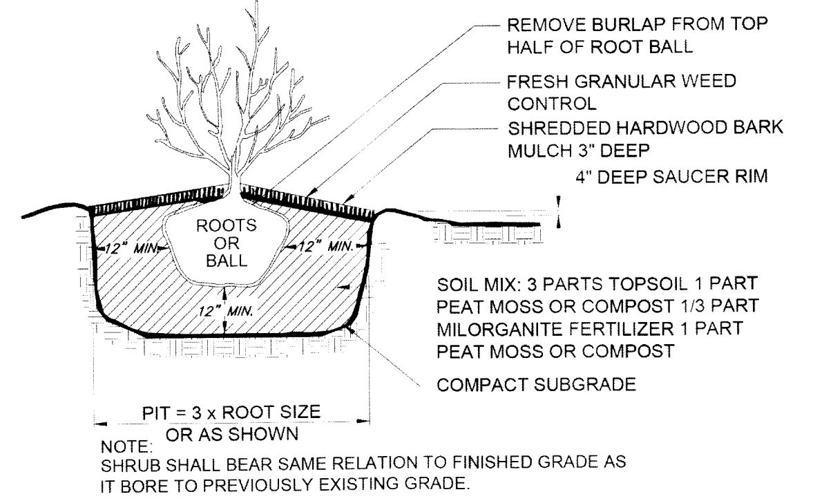
3 SHRUB PLANTING DETAIL SCALE: NO SCALE
