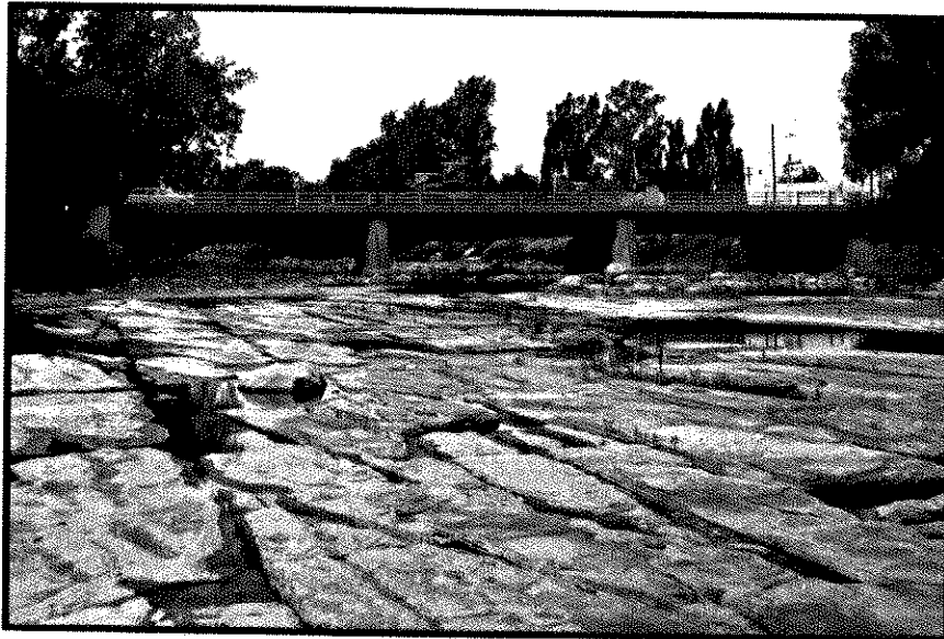
Photo No. 20. Looking downstream at Transit Road bridge showing the rock channel bottom.
