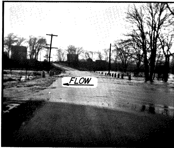
Photo No. 6. Looking north along Borden Road during the March 1955 flood. Although water is over the road the bridge, shown in the background, is not full. This is looking in the opposite direction from photos 4 and 5.
