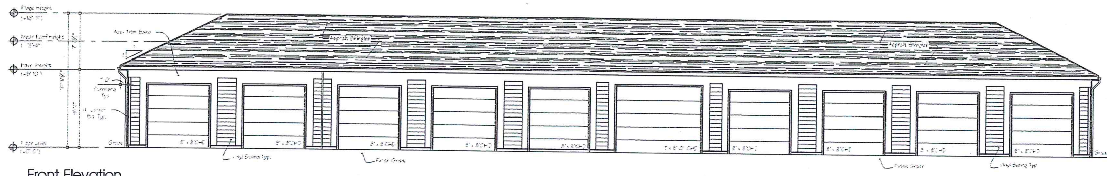
Front Elevation
