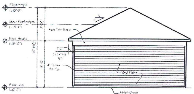
Side Elevation
